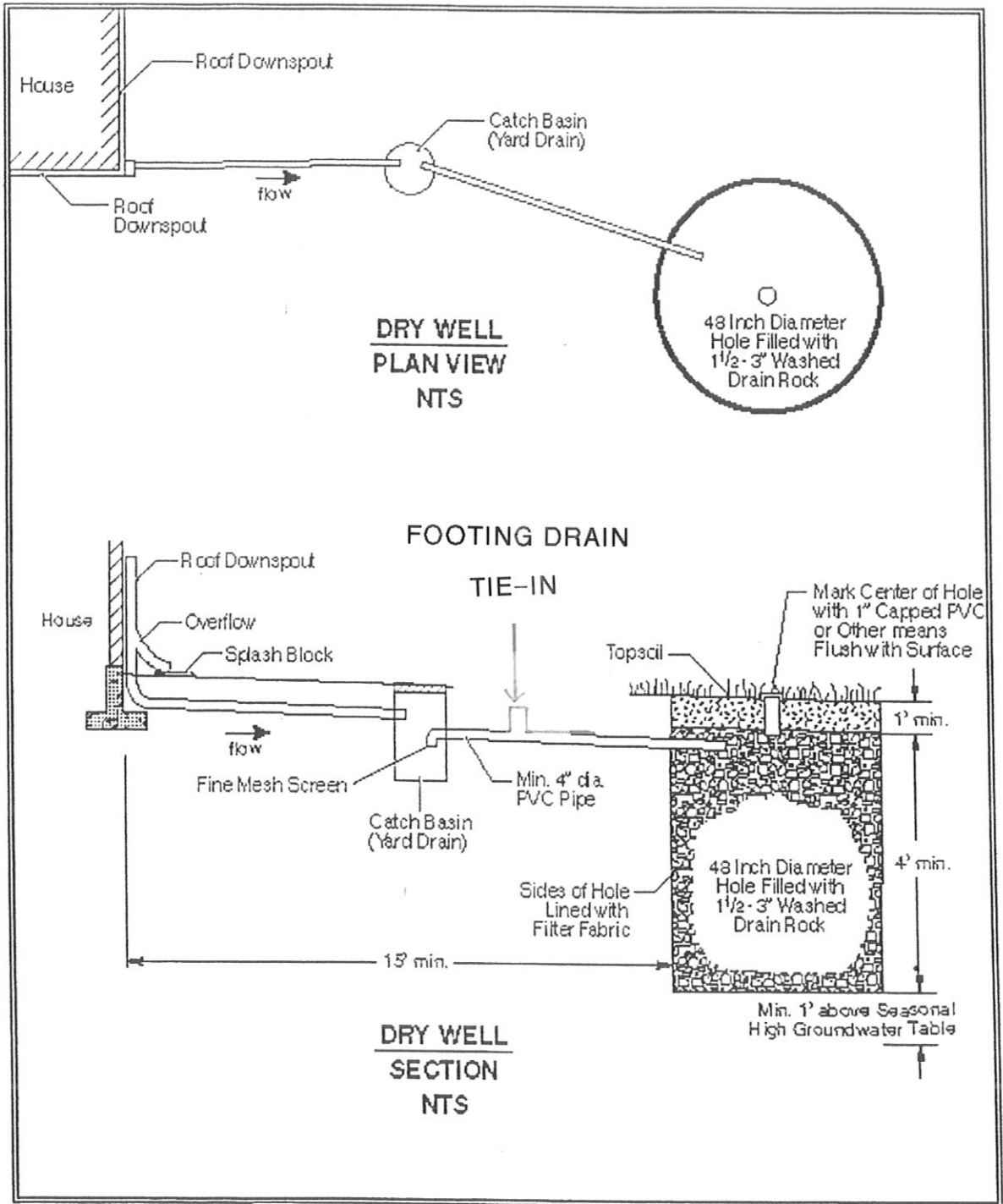
DRYWELL SYSTEM
